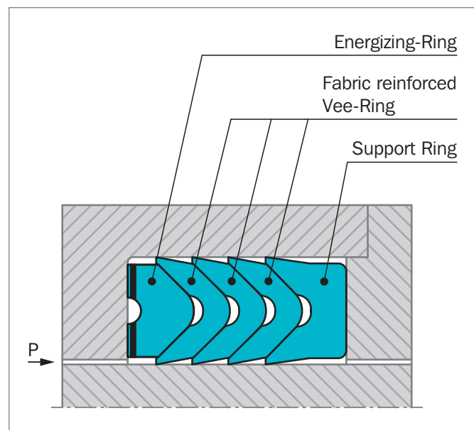
Figure 31: Veepac design with 3 fabric reinforced vee-ring
