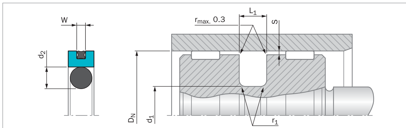
Figure 124: Installation Drawing
