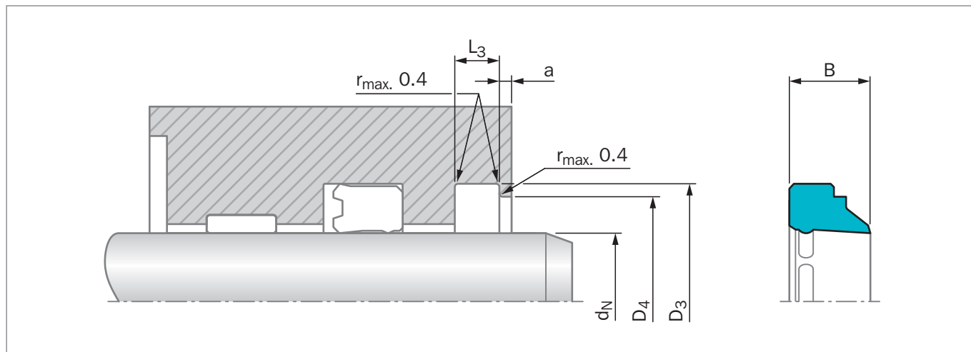
Figure 189: Installation Drawing
