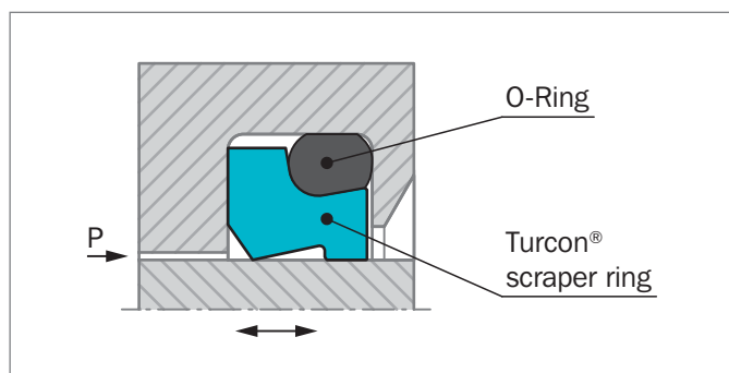
Figure 164: Turcon® Excluder® 5
