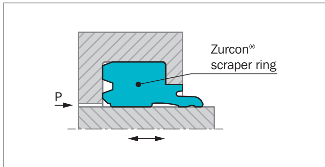
Figure 192: Scraper WNV
