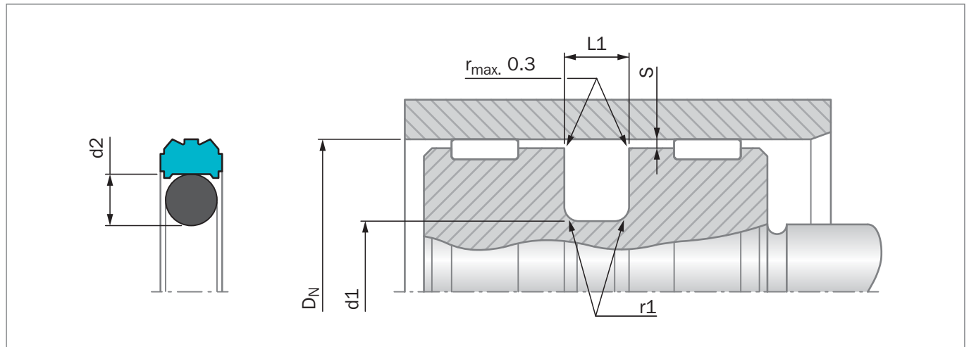
Figure 144: Installation Drawing
