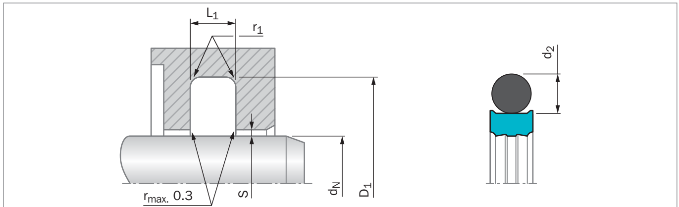
Figure 90: Installation Drawing
