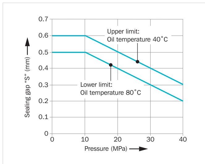
Figure 58: Radial clearance "S" as function of pressure
