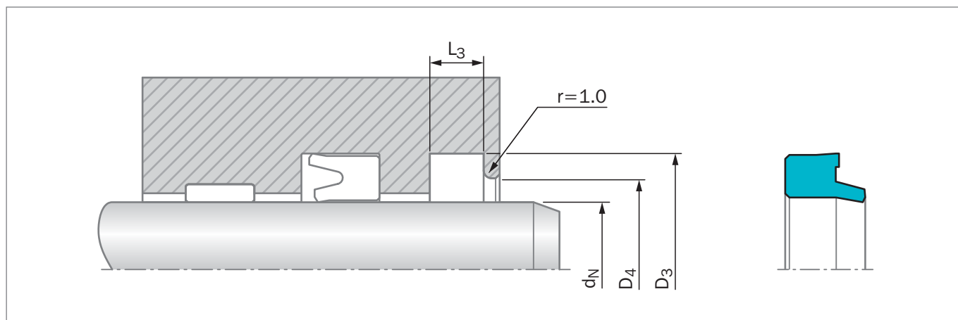
Figure 191: Installation Drawing
