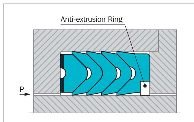
Figure 32: Veepac design with anti-extrusion ring
