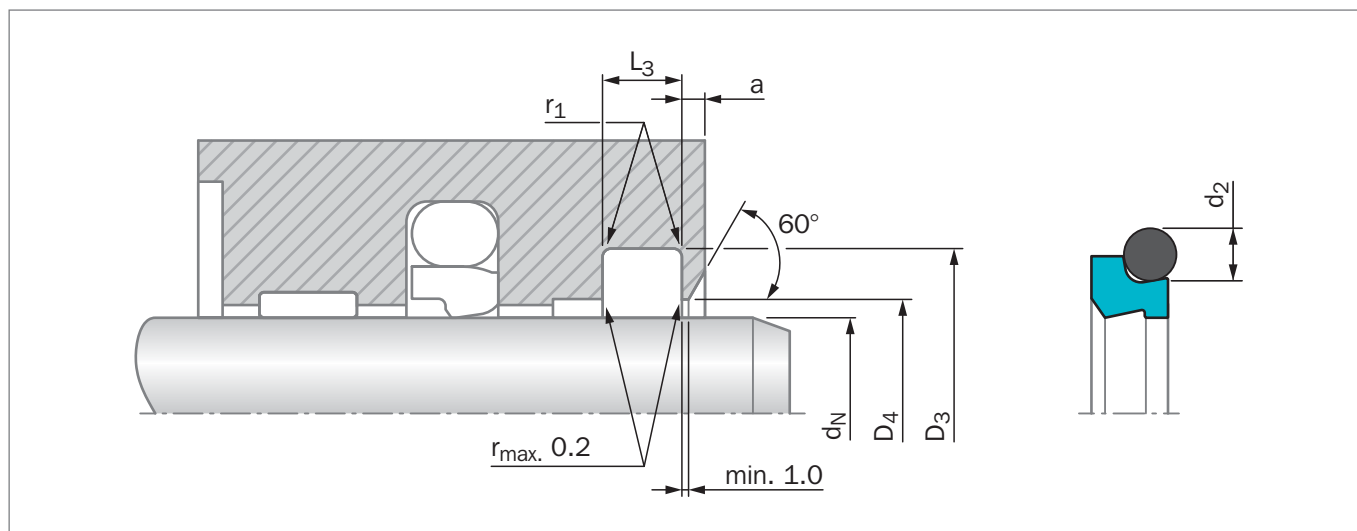
Figure 165: Installation Drawing
