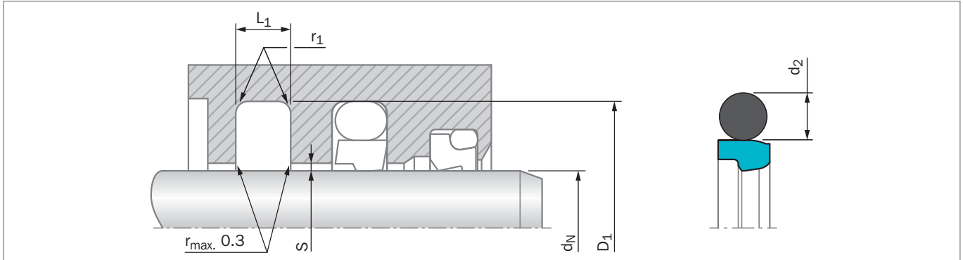
Figure 22: Installation Drawing
