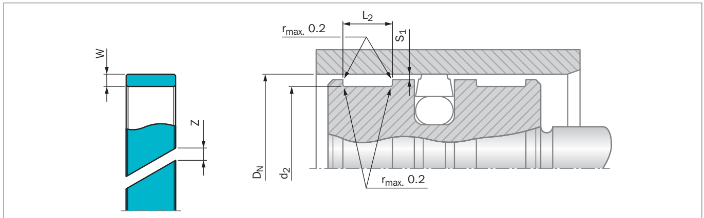
Figure 211: Installation Drawing
