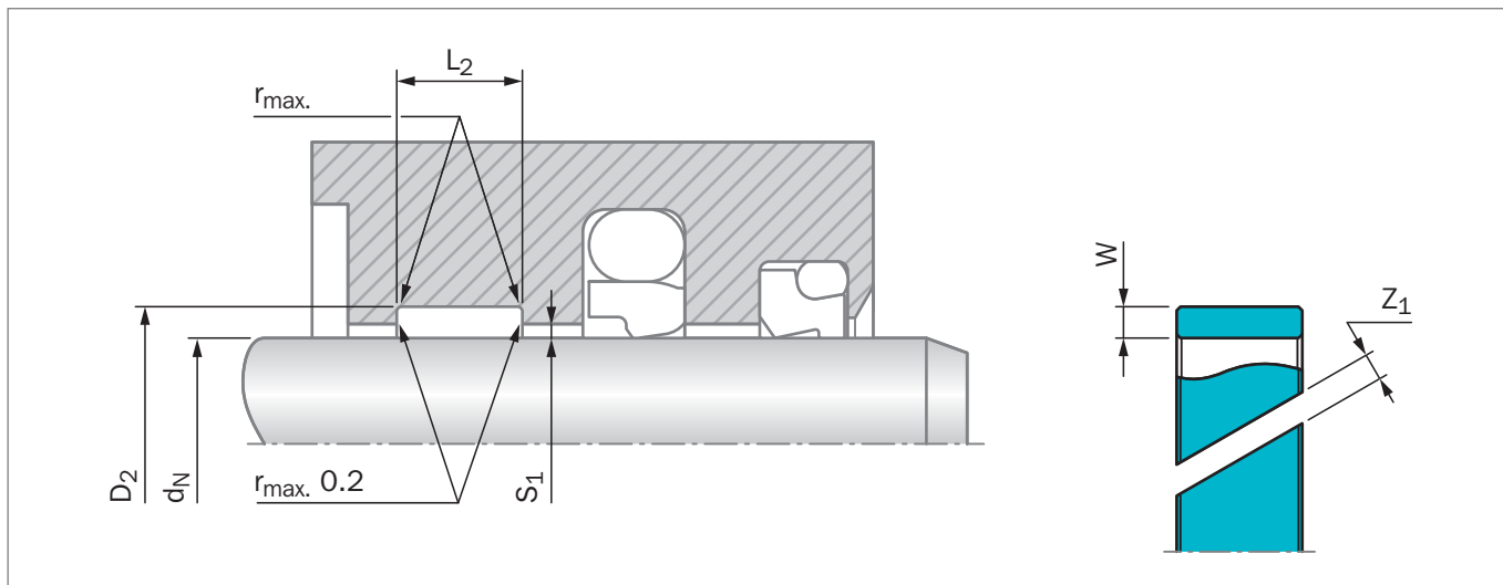
Figure 215: Installation Drawing
