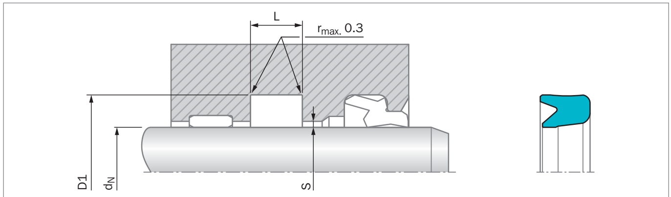
Figure 59: Installation Drawing, Dimension "S" see Figure 58
