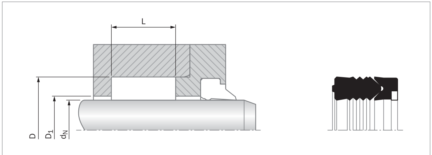
Figure 38: Installation Drawing
