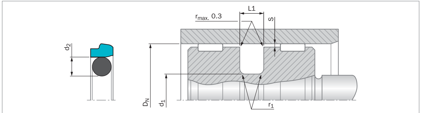
Figure 126: Installation Drawing
